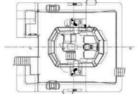
Bridge deck
